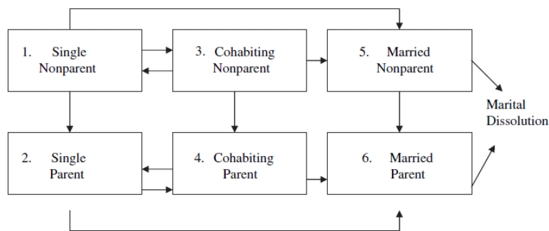
FIGURE 2. DIAGRAM OF THE FULL SIX LIVING STATE MULTISTATE MODEL OF FAMILY TRANSITIONS.
